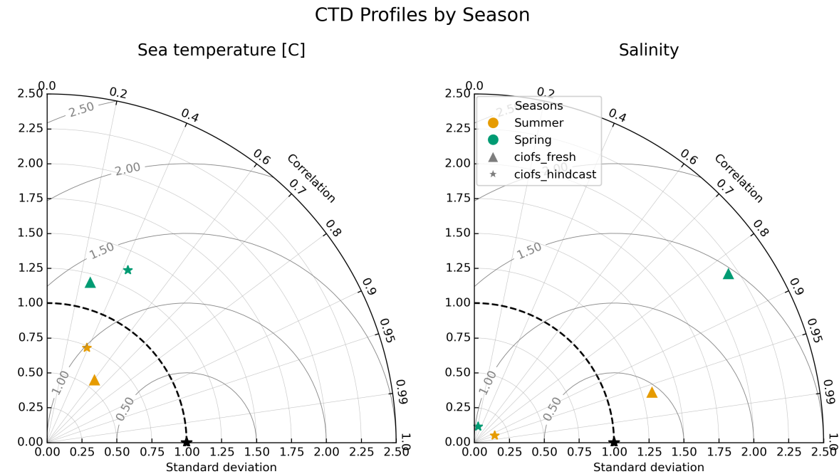
Fig. 4 Taylor Diagram summarizing skill of CIOFS Hindcast (stars) and CIOFS Fresh (triangles) for temperature (left) and salinity (right), grouped by season, for CTD profiles datasets.
