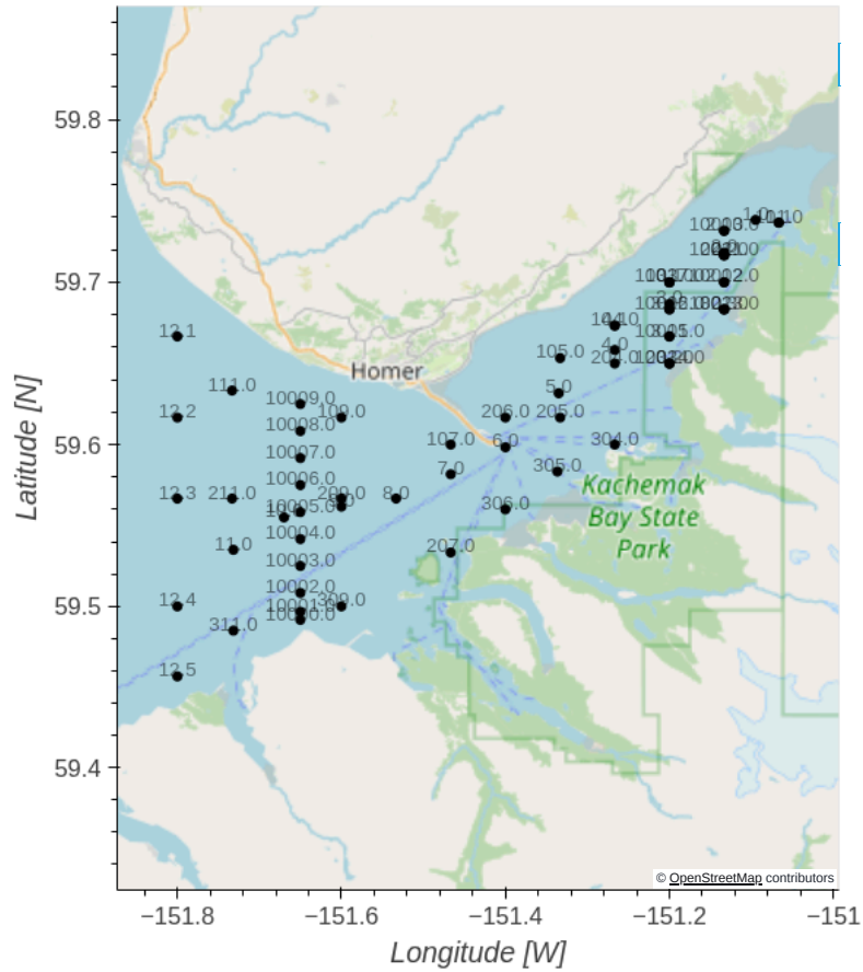
ctd_profiles_kachemack_kuletz_2005_2007
