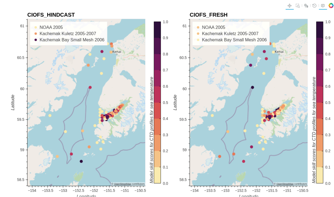
Fig. 5 Skill scores for CIOFS Hindcast (left) and CIOFS Freshwater (right) with CTD profiles for sea temperature, by project. Click on a legend entry to toggle the transparency. (HTML plot, won't show up correctly in PDF.)
