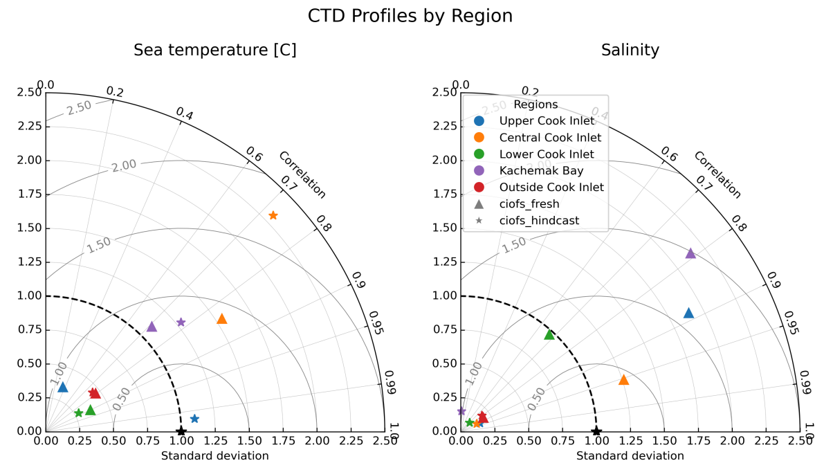
Fig. 3 Taylor Diagram summarizing skill of CIOFS Hindcast (stars) and CIOFS Fresh (triangles) for temperature (left) and salinity (right), grouped by region of Cook Inlet, for CTD profiles datasets.
