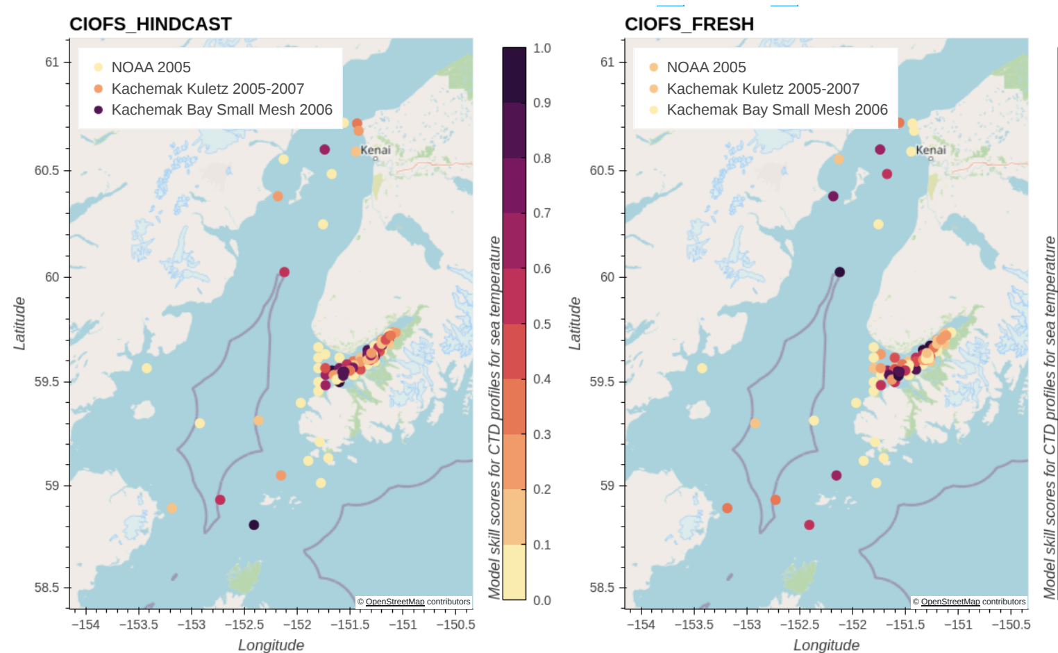
Fig. 5 Skill scores for CIOFS Hindcast (left) and CIOFS Freshwater (right) with CTD profiles for sea temperature, by project. Click on a legend entry to toggle the transparency. (HTML plot, won't show up correctly in PDF.)
